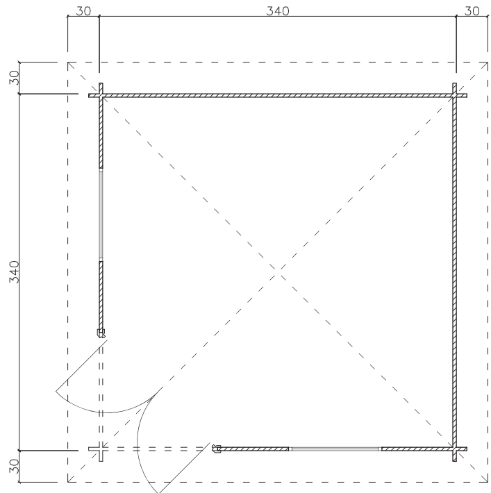
Grundriss / ground plan plattegrond / plan / rzut
