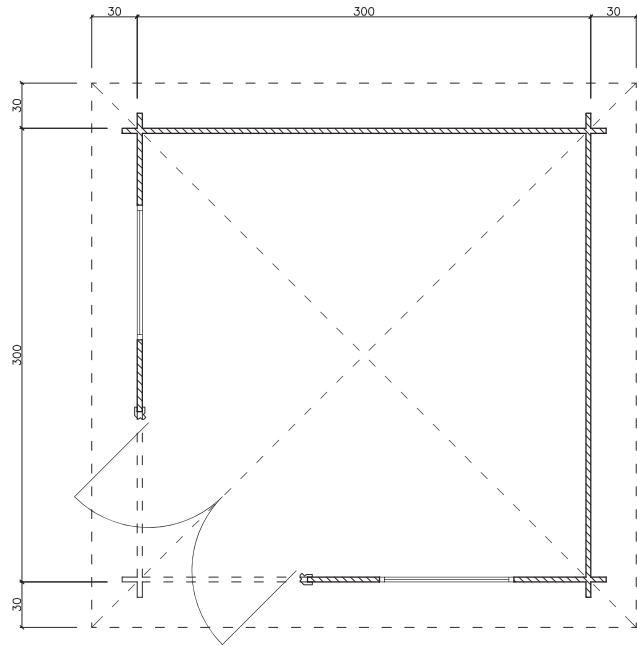
Grundriss / ground plan plattegrond / plan / rzut
