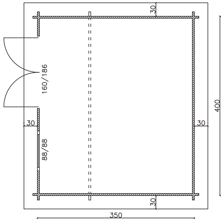
Grundriss / ground plan / plattegrond / plan / rzut
